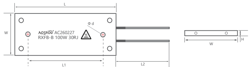
RXFB-B 超薄云母板线绕电阻器 RXFB-B Thin Mica Plate Wire Wound Resistor
