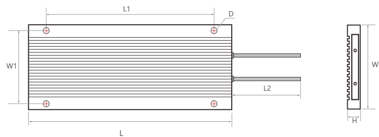
RXFB 产品尺寸图 (RXFB Product Size)
