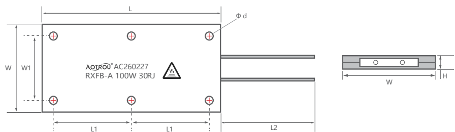
RXFB-A 产品尺寸图 (RXFB-A Product Size)
